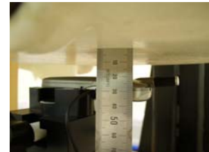
Fig. 22. Body SAR Test Setup with Holster
