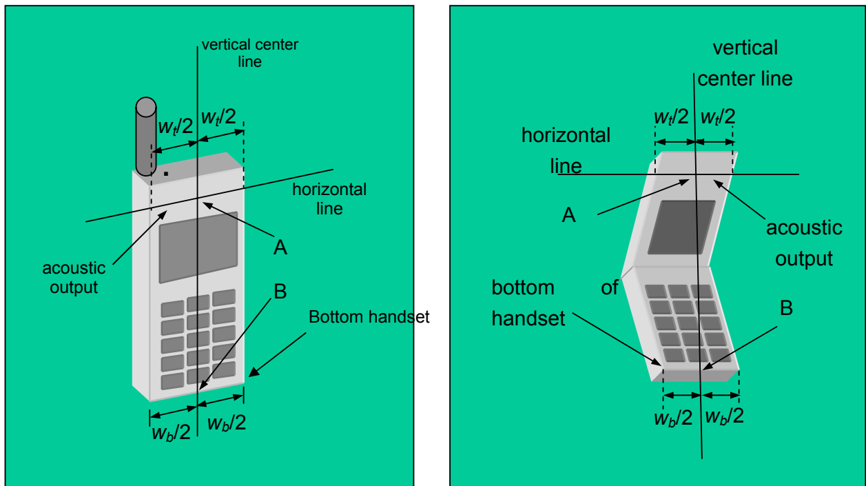
Figure 7. Device Test Position
