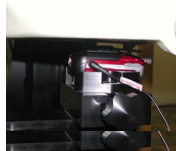
Fig. 20. Body SAR Test Setup with Holster
