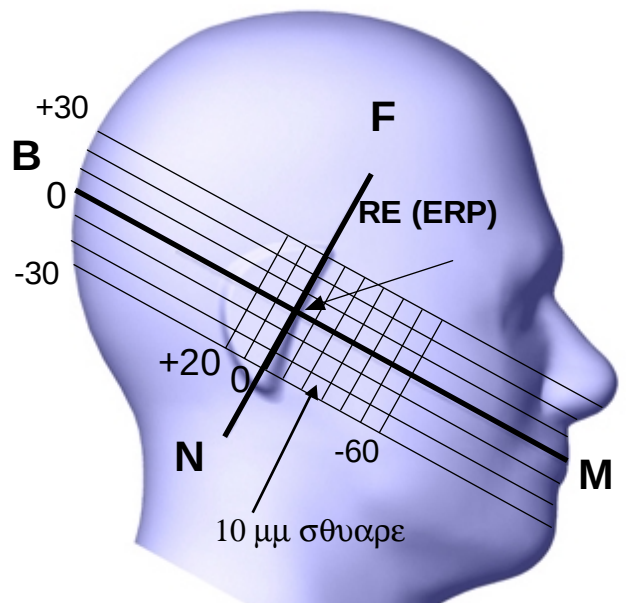
Figure 6. EUT Head Position
