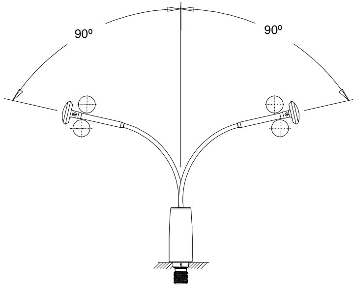
Figure 4. Method for Whip Bending Endurance Testing
