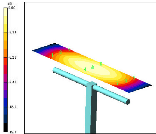
0 dB = 0.283A/m
