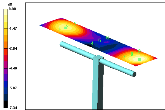
0 dB = 147.1V/m
