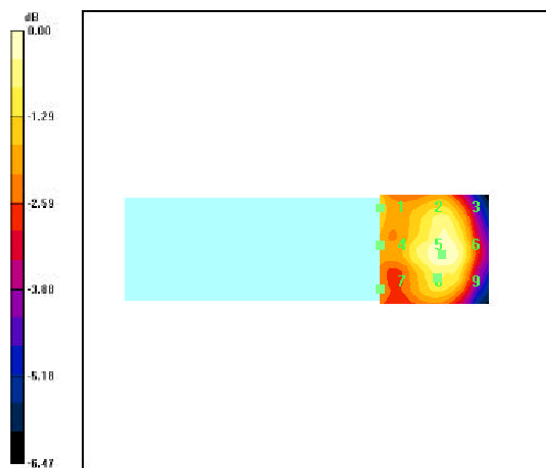
0 dB = 47.7V/m
