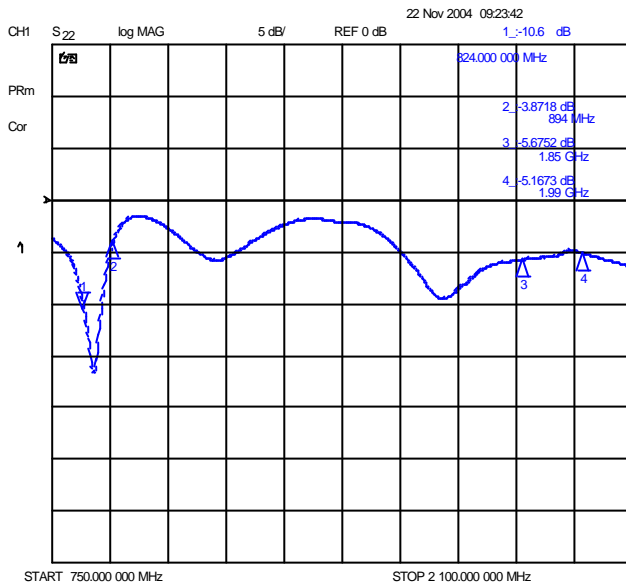
Return Loss Antenna Retracted Flip Open
