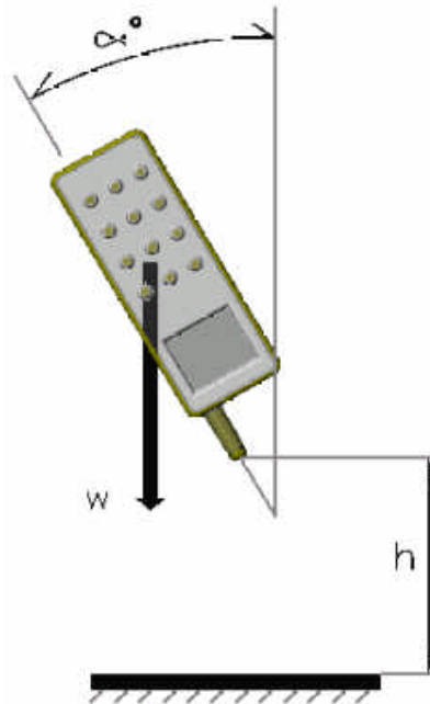
Figure 3-6: Drop test
