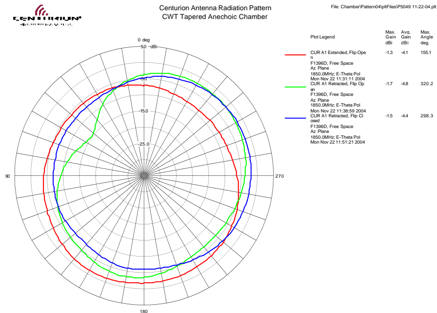
Figure 2-11: OPEN EXTENDED /OPEN & CLOSE RETRACTED PCS (1850 MHz) – Az
