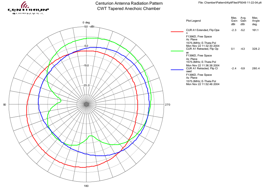
Figure 2-10: OPEN EXTENDED /OPEN & CLOSE RETRACTED GPS (1575 MHz) – Az
