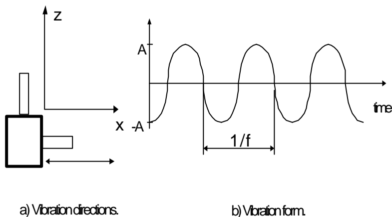
Figure 4-2: Sinusoidal Vibration
