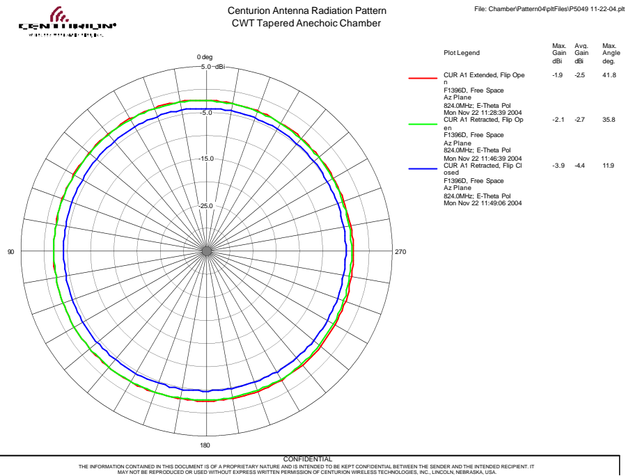
Figure 2-6: OPEN EXTENDED /OPEN & CLOSE RETRACTED CDMA (824 MHz) – Az
