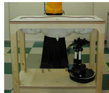
Figure 11. SAM Phantom
