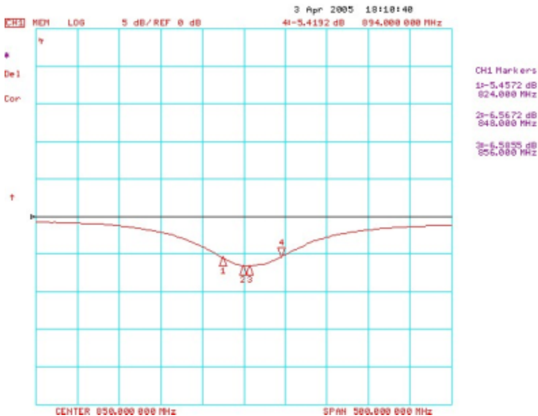
Figure6. Return loss
