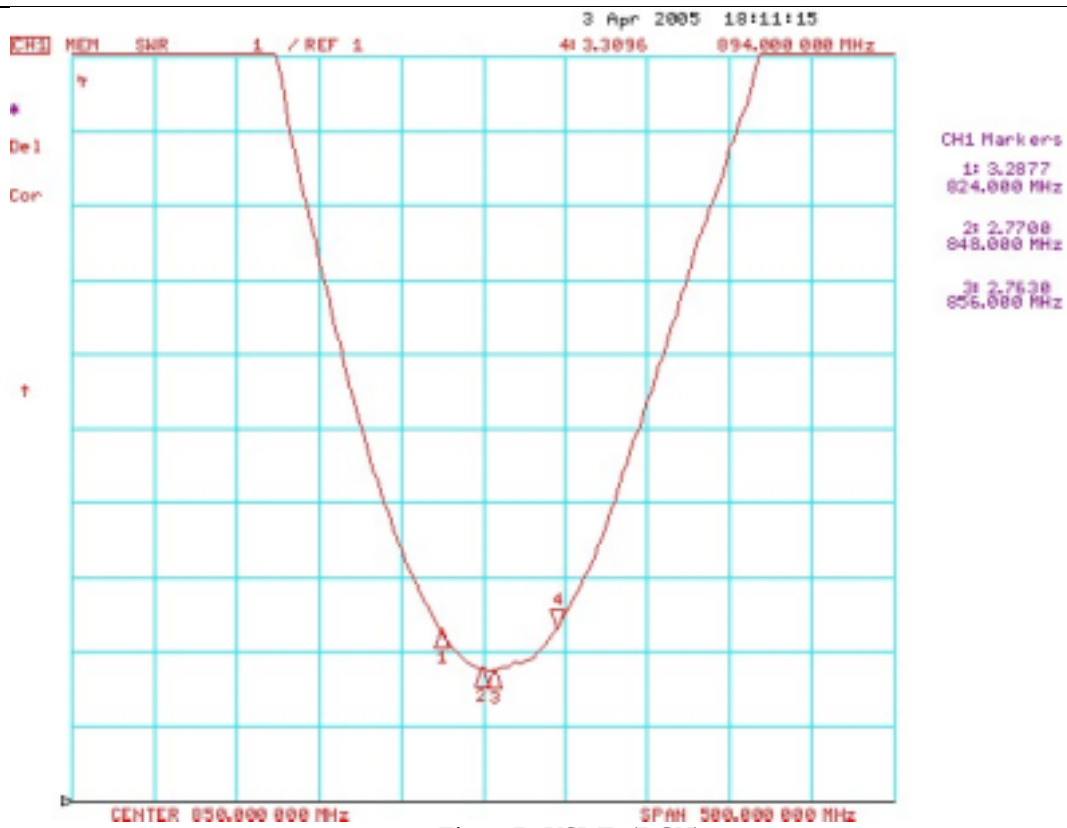
Figure7. VSWR (DCN)
