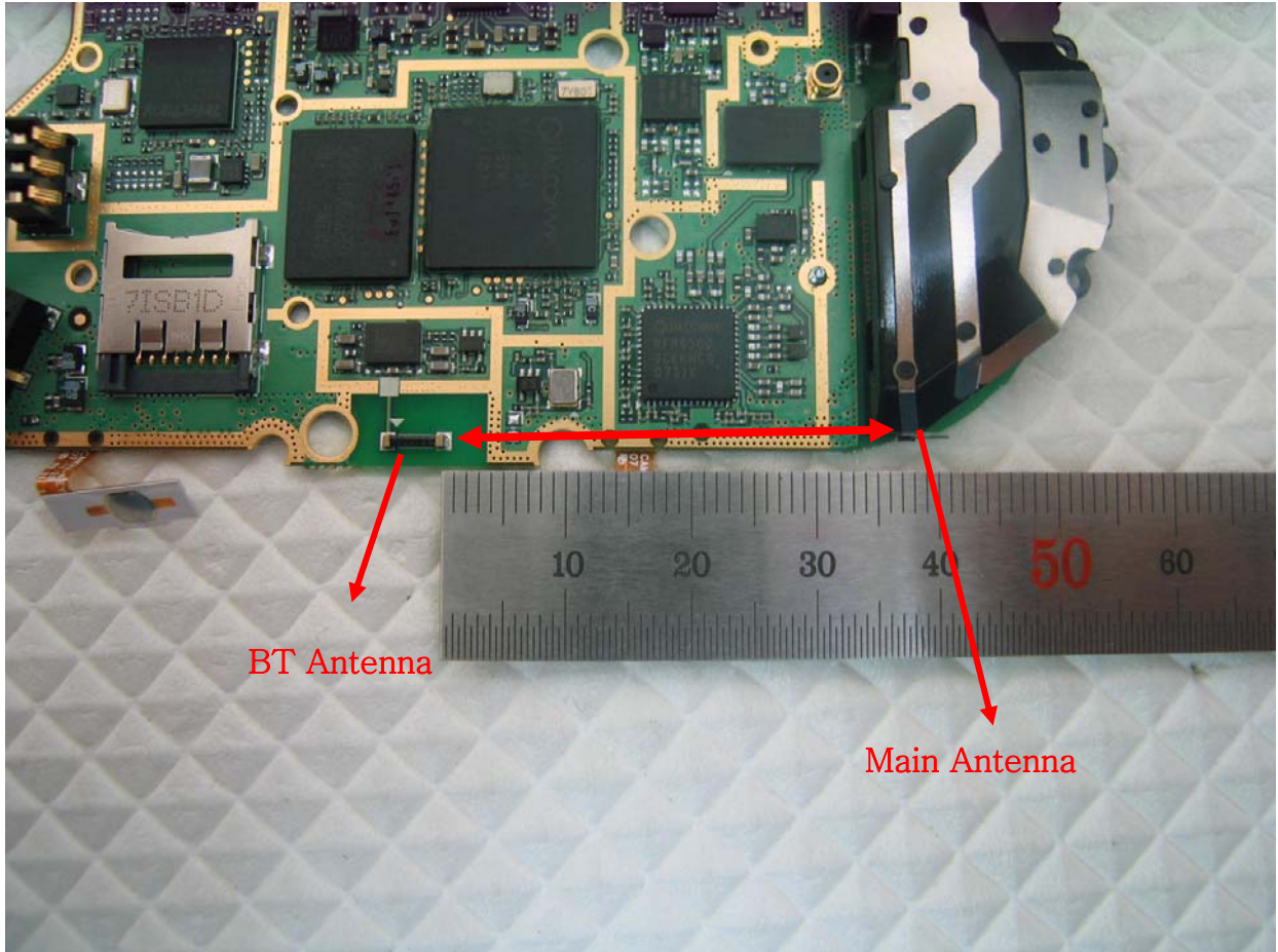
[Antenna separation distance: 3.7 cm]
