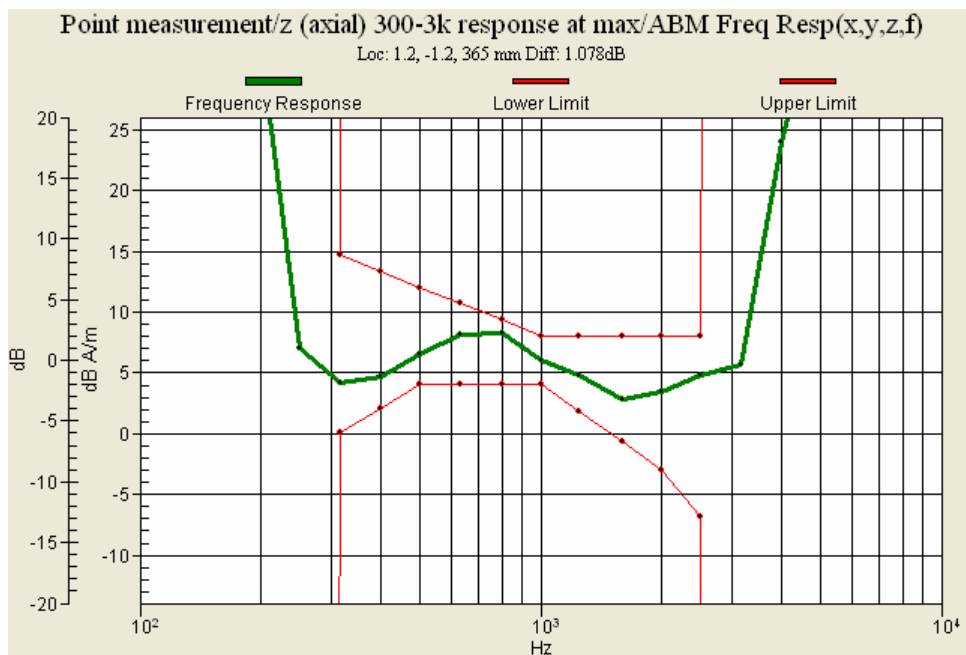
Figure 14 : PCS CDMA (CH 25) Frequency Response (Slide down)
