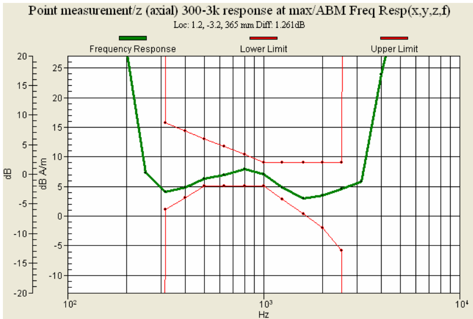
Figure 17 : CDMA (CH 1013) Frequency Response (Slide up)
