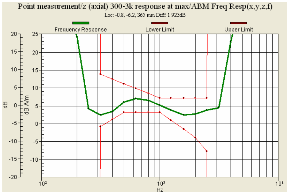
Figure 18 : CDMA (CH 384) Frequency Response (Slide up)
