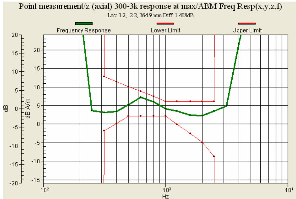
Figure 12 : CDMA (CH 384) Frequency Response (Slide down)
