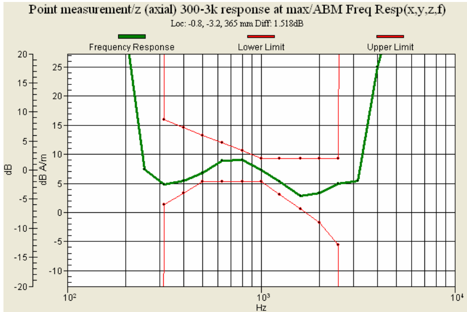
Figure 11 : CDMA (CH 1013) Frequency Response (Slide down)
