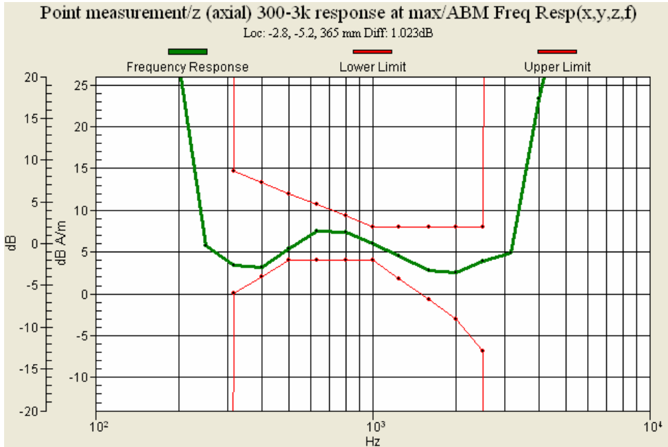
Figure 15 : PCS CDMA (CH 600) Frequency Response (Slide down)
