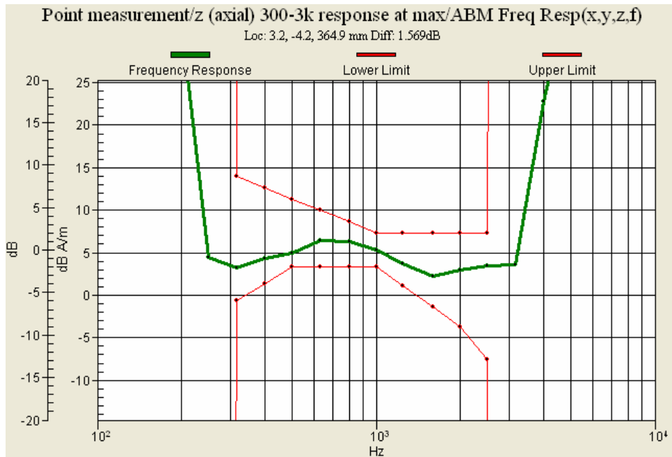
Figure 13 : CDMA (CH 777) Frequency Response (Slide down)
