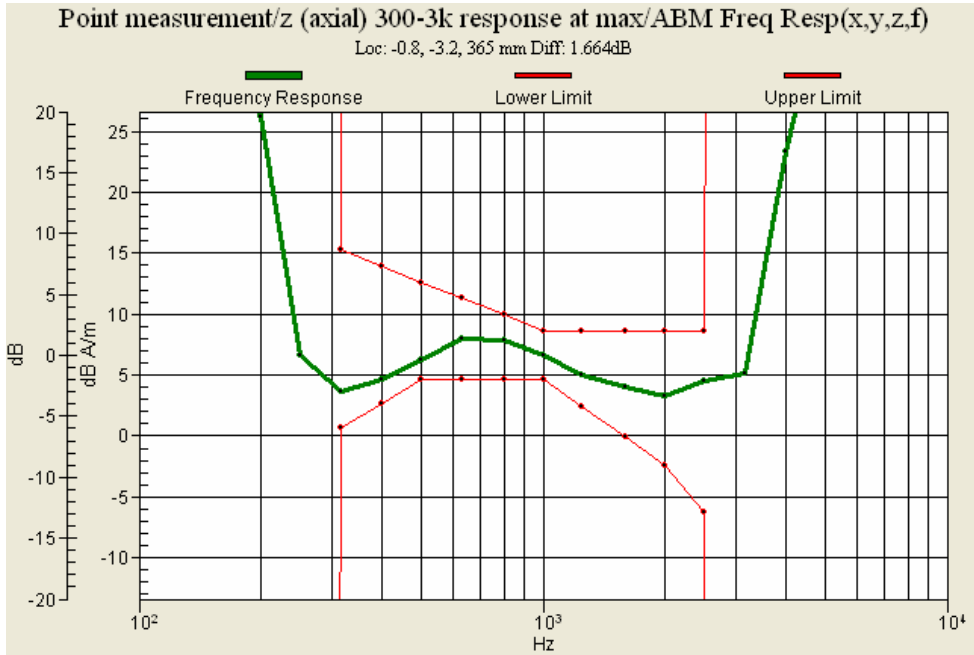
Figure 21 : PCS CDMA (CH 600) Frequency Response (Slide up)
