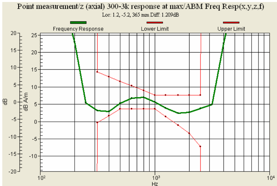
Figure 20 : PCS CDMA (CH 25) Frequency Response (Slide up)
