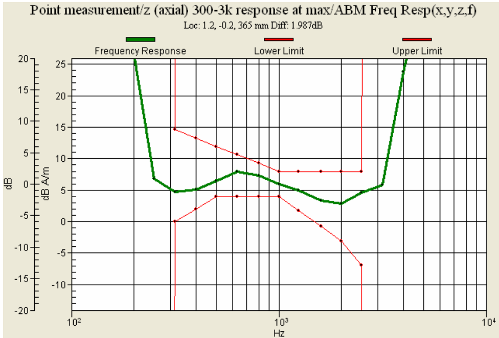
Figure 19 : CDMA (CH 777) Frequency Response (Slide up)
