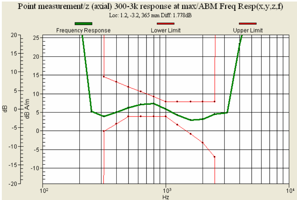
Figure 16 : PCS CDMA (CH 1175) Frequency Response (Slide down)
