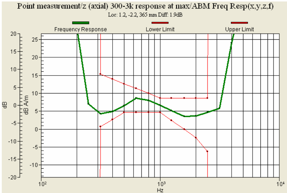
Figure 22 : PCS CDMA (CH 1175) Frequency Response (Slide up)
