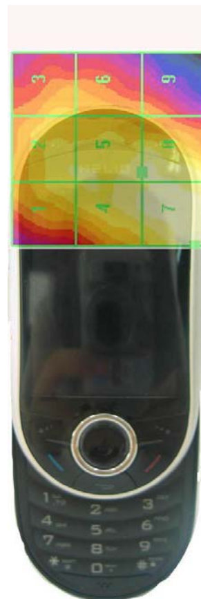
H-Field WD Scan overlay
