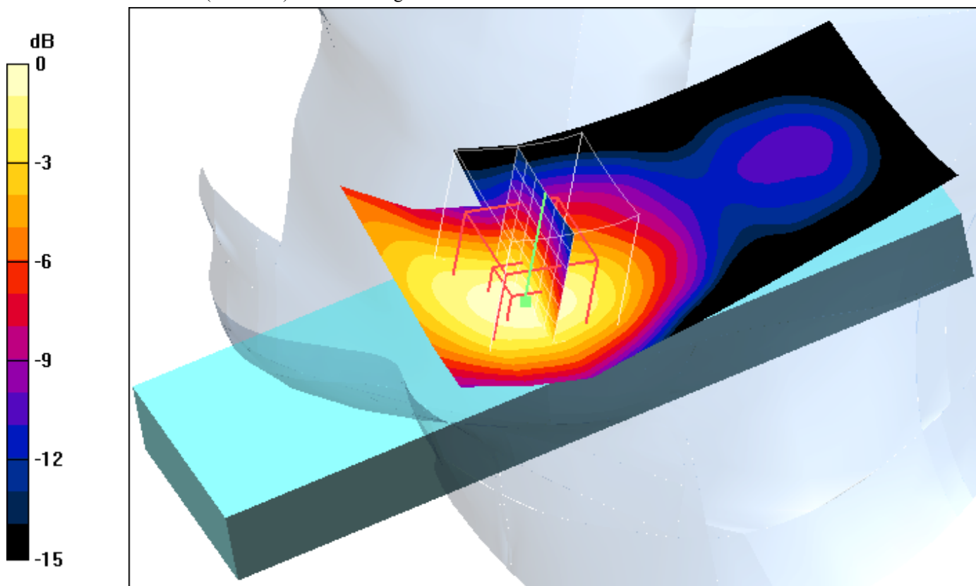
0 dB = 0.748mW/g
