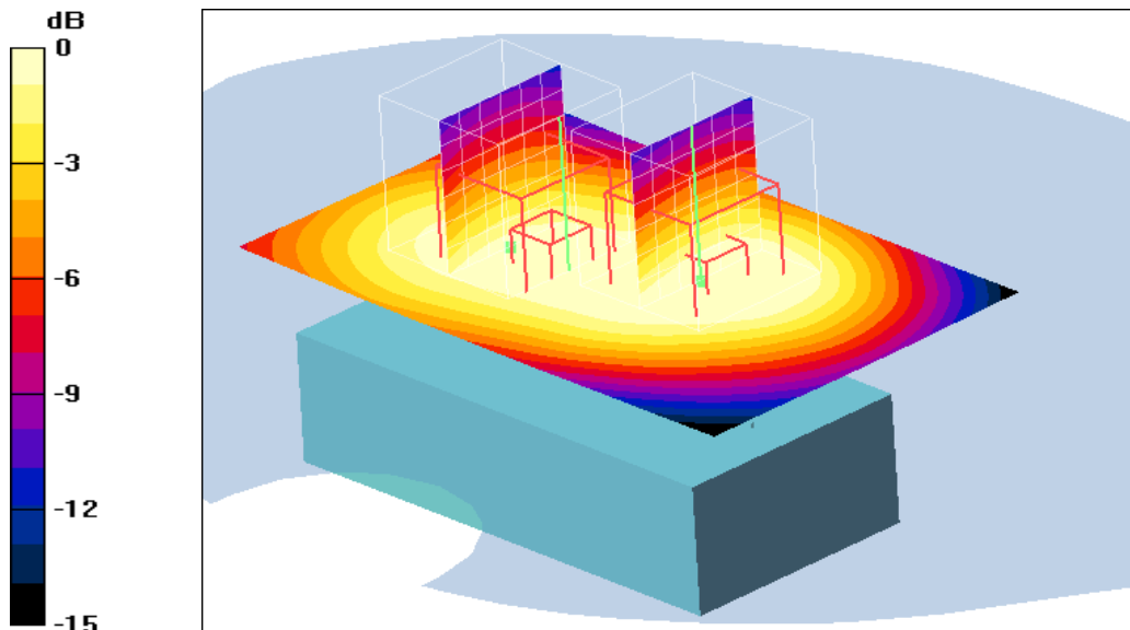
0 dB = 0.405mW/g
