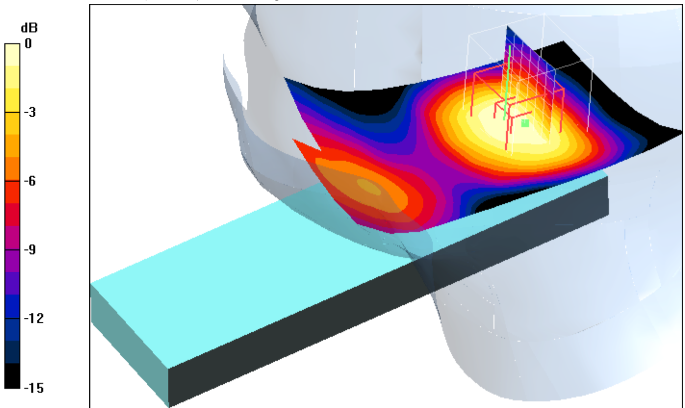
0 dB = 0.232mW/g
