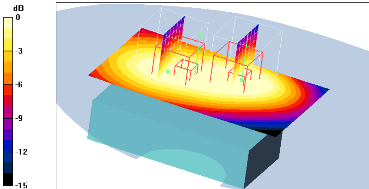
0 dB = 0.292mW/g
