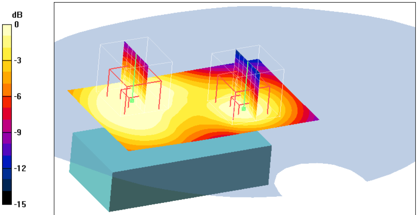
0 dB = 0.180mW/g
