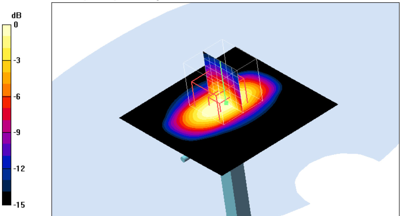
0 dB = 46.4mW/g
