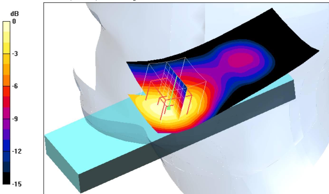
0 dB = 0.671mW/g
