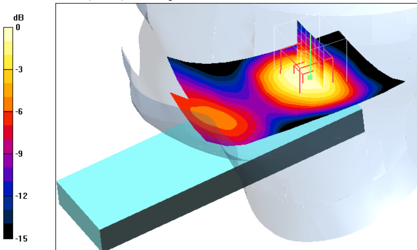
0 dB = 0.257mW/g
