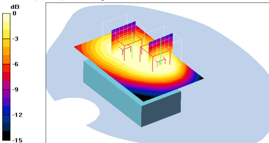
0 dB = 0.338mW/g
