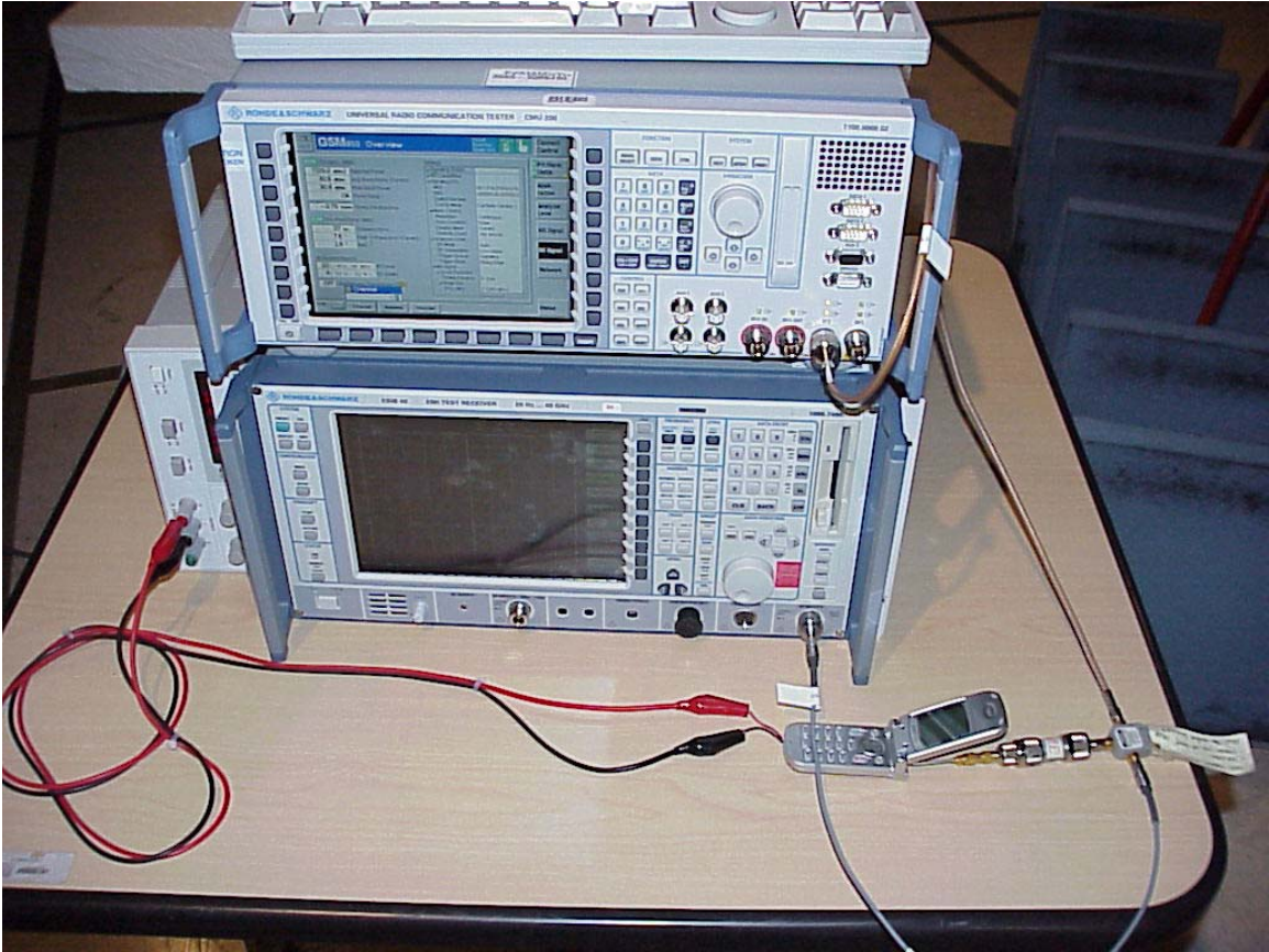
Test setup for Mobile Emissions in base band for FCC ID: PP4GA-160C
