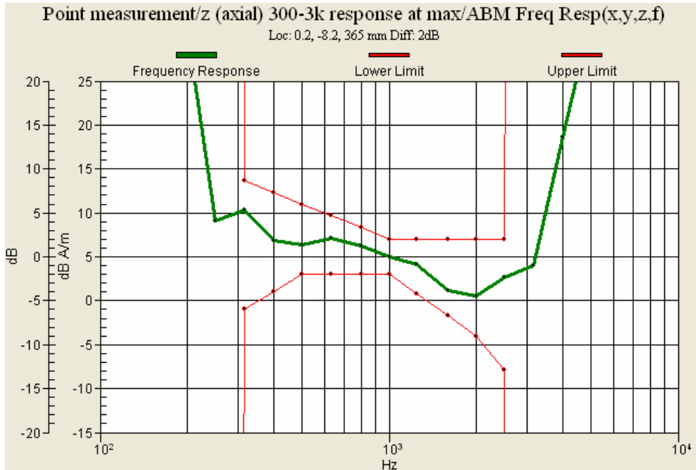
Figure 11 : CDMA (CH 1013) Frequency Response
