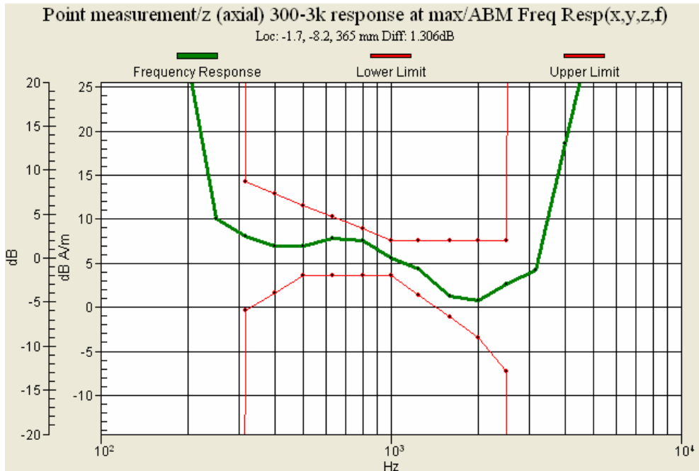
Figure 12 : CDMA (CH 384) Frequency Response
