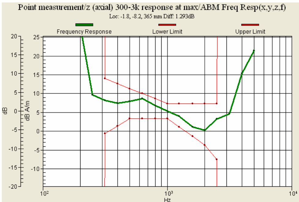
Figure 16 : PCS CDMA (CH 600) Frequency Response
