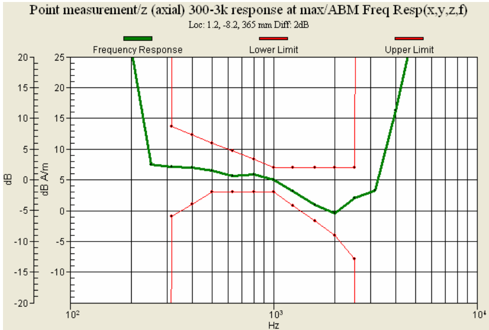
Figure 15 : PCS CDMA (CH 25) Frequency Response
