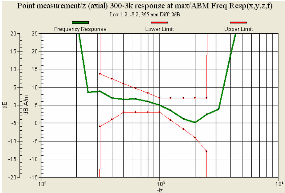
Figure 13 : CDMA (CH 777) Frequency Response
