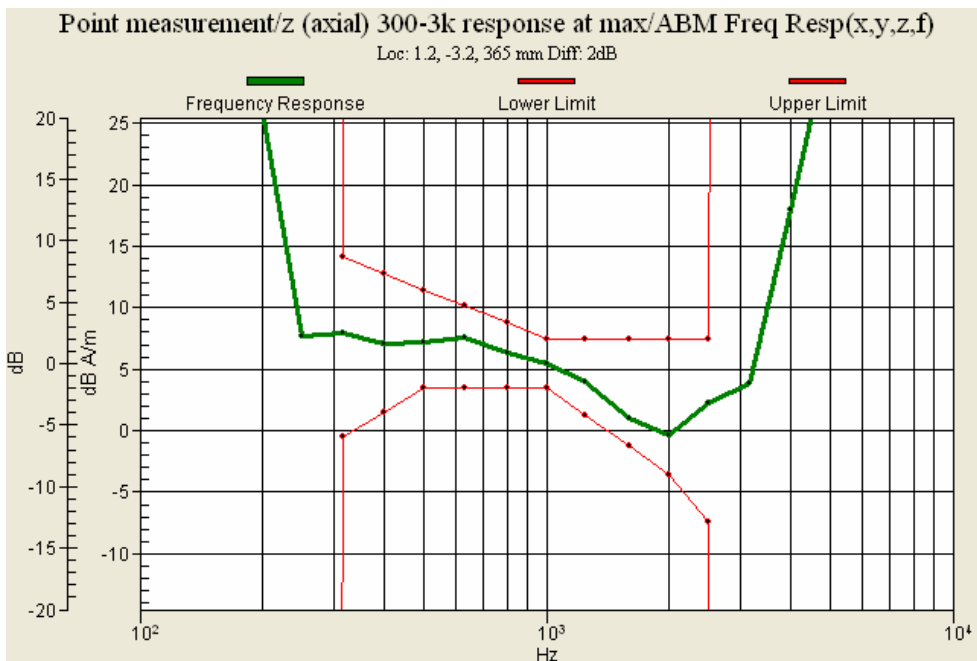
Figure 14 : CDMA (CH 384) Frequency Response (T-coil Center)
