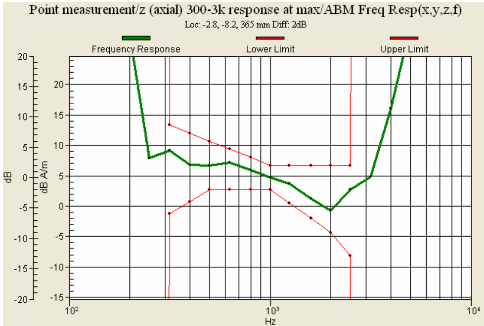
Figure 17 : PCS CDMA (CH 1175) Frequency Response
