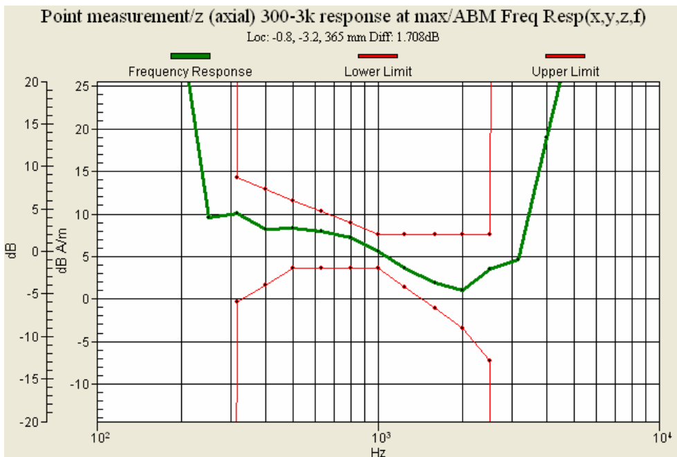
Figure 18 : PCS CDMA (CH 600) Frequency Response (T-coil Center)
