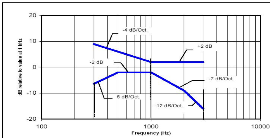
Figure 5 : Magnetic field frequency response for WDs with a field that exceeds - 10 dB(A/m) at 1 kHz
