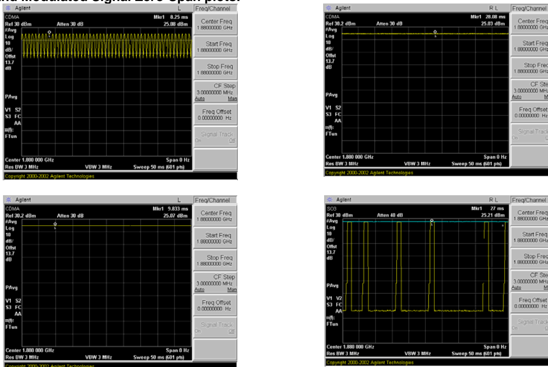
Figure 8-4 Zero-Span Plots
