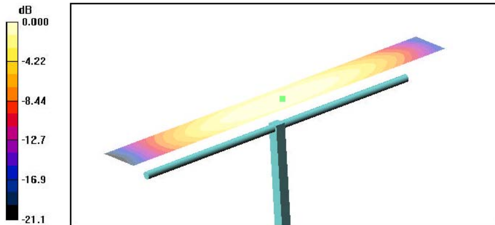
0 dB = 0.463A/m
