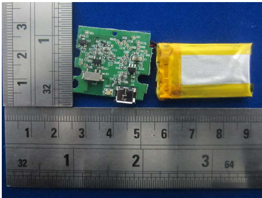
EUT –Main Board With Battery Bottom View
