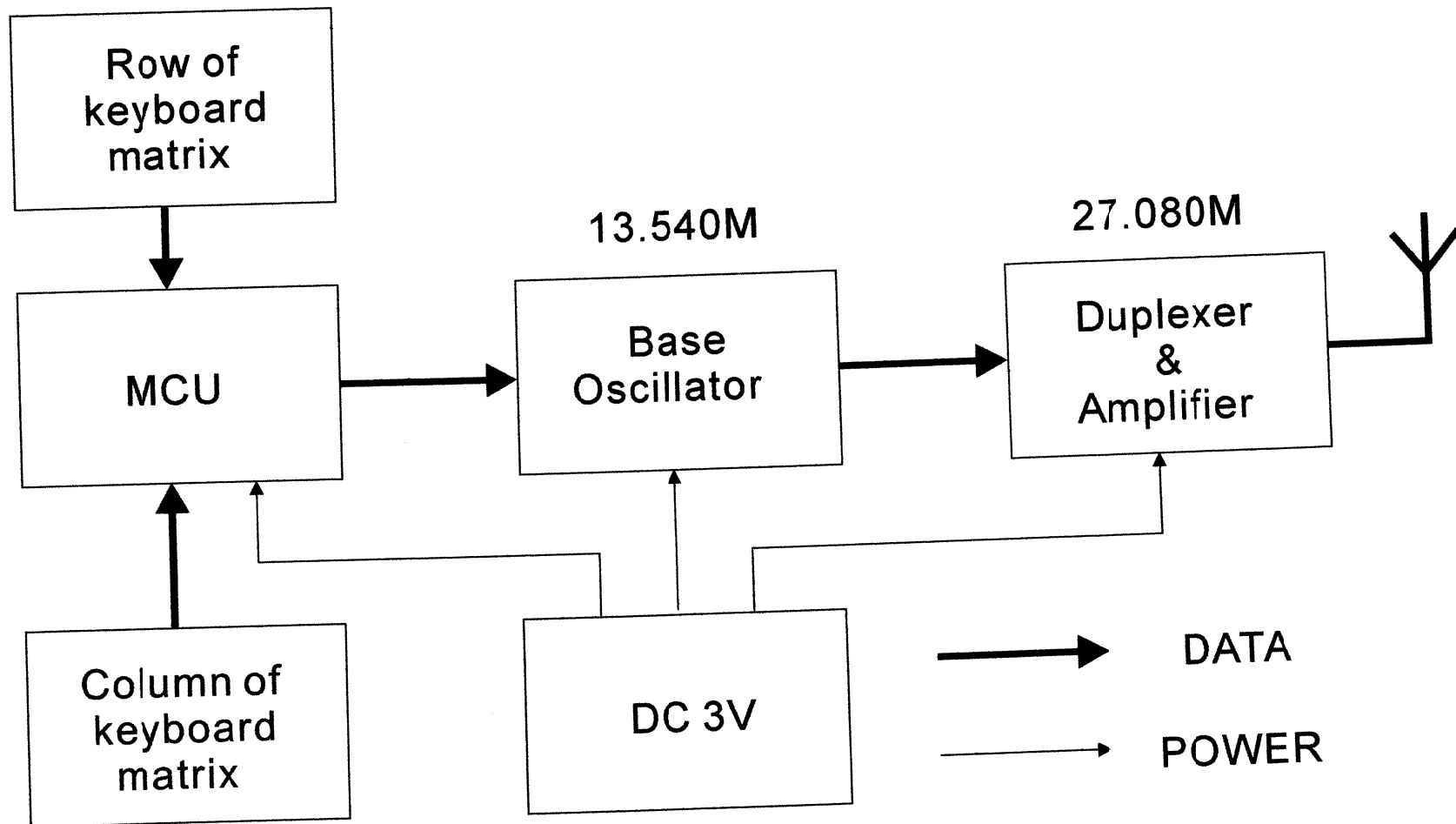
Cordless Keyboard Block Diagram
