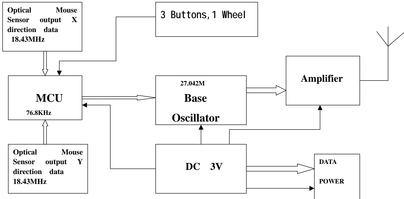
Note: 18.43MHz use optical mouse sensor; 76.8KHz use MCU; 27.042 use transmit Oscillator Wireless Optical Mouse Block Diagram
