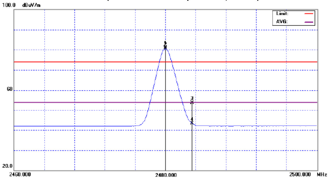
TX CH 16 (Restricted Bands Requirements, Vertical)
