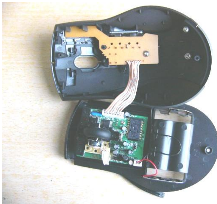
Main & RF board component side
