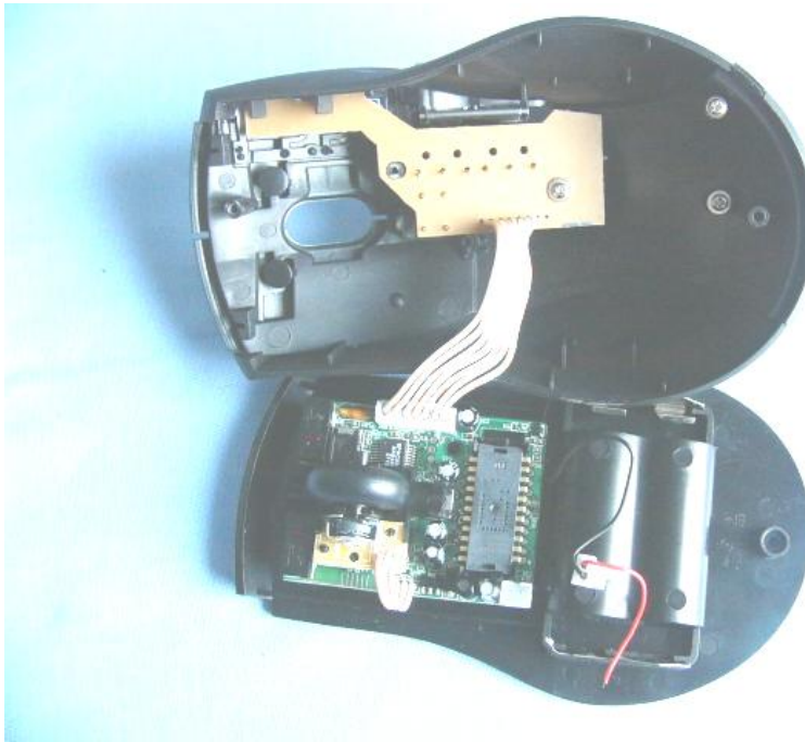
Main & RF board component side
