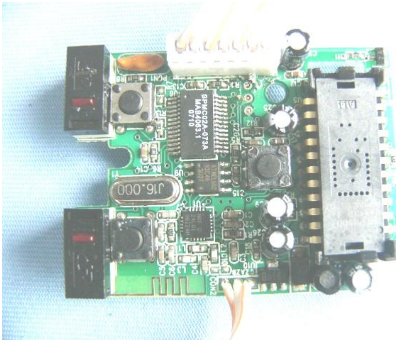
Main & RF board component side
