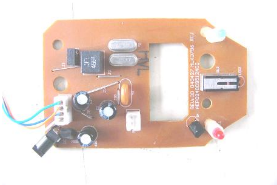
Rx board solder side
