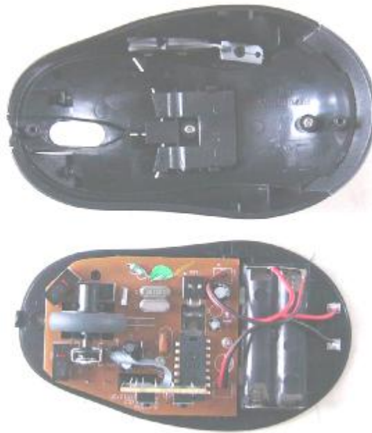
Main board component side
