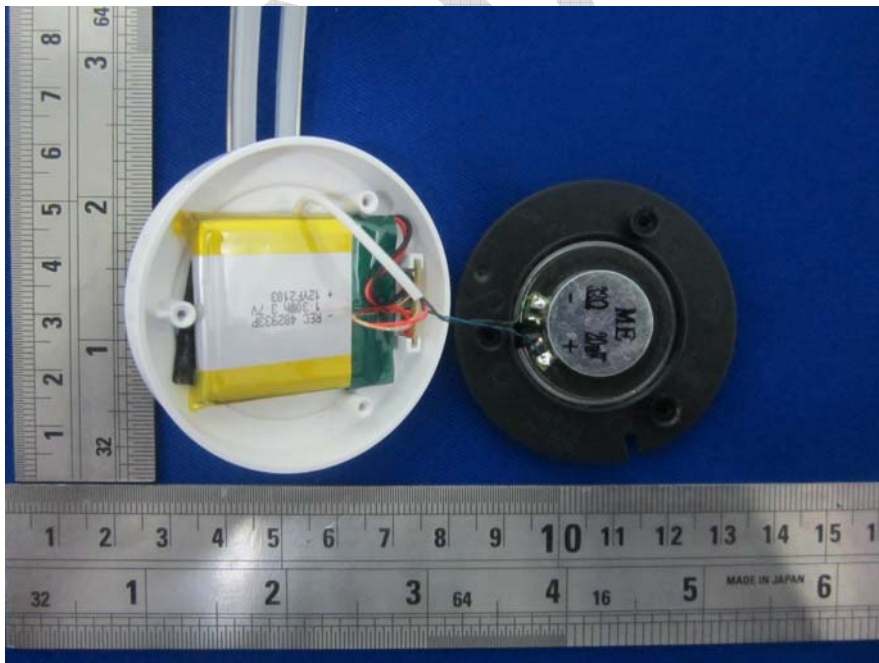
EUT- Right Headset Uncover View
