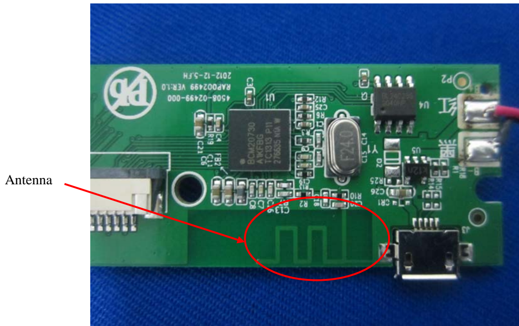
EUT –Chip and Antenna View
