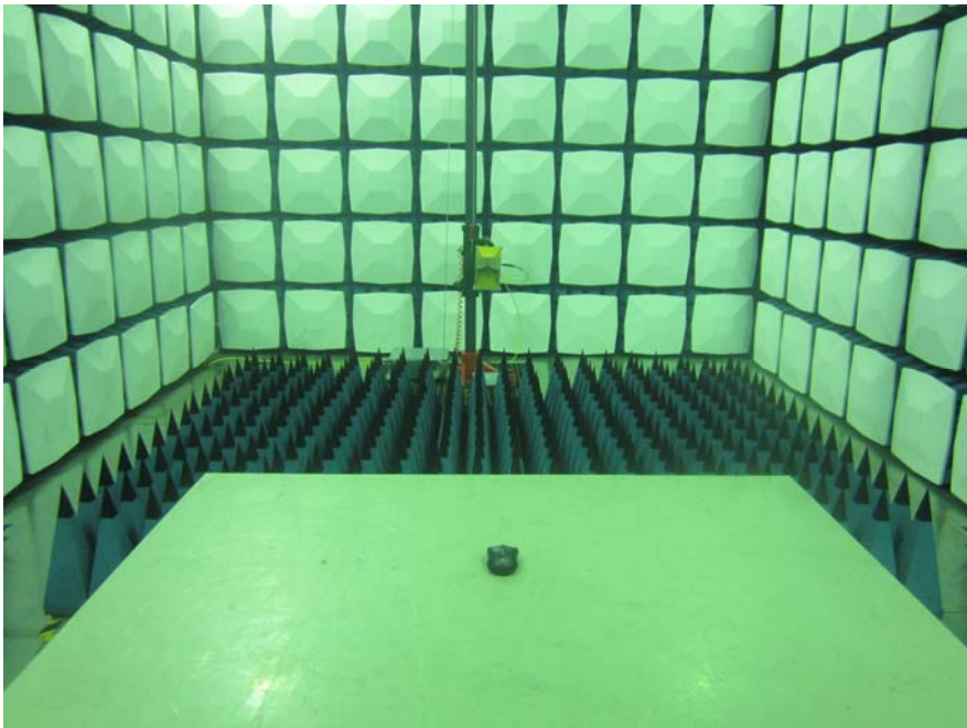
Radiated Emissions Above 1G View
