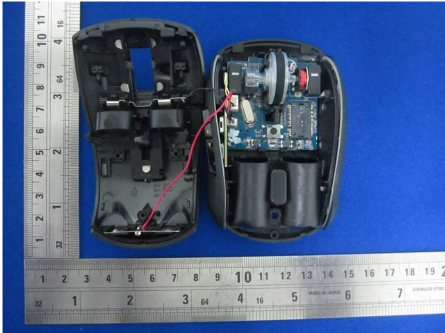
EUT – Top Cap View
