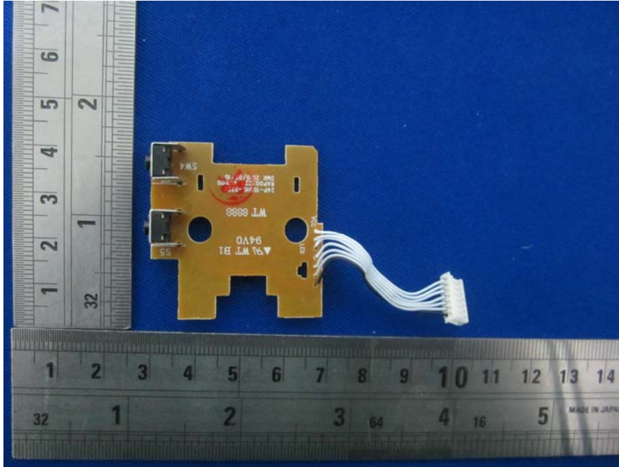
EUT – Button PCB Board Top View
