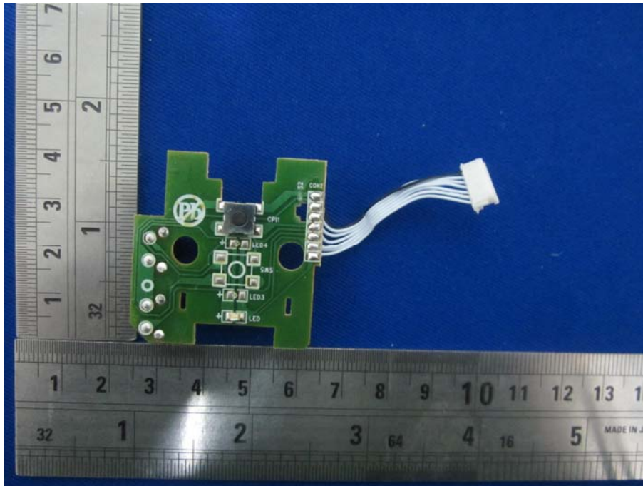
EUT –Button PCB Board Bottom View
