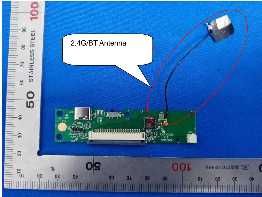
VIEW OF EUT (FIGURE 1)
