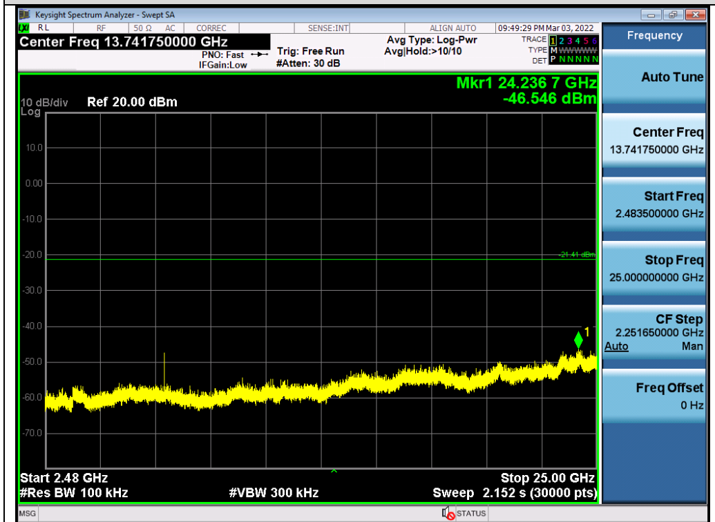
Test_Graph_2.4GHz_ANT1_2446_GFSK_Higher Band Emissions
