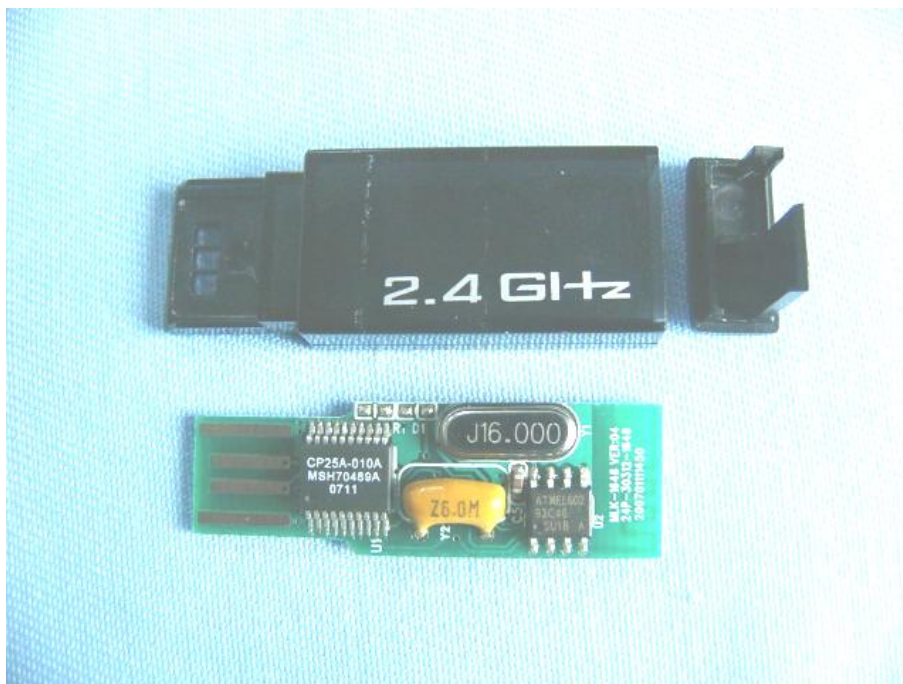
Rx Main board component side
