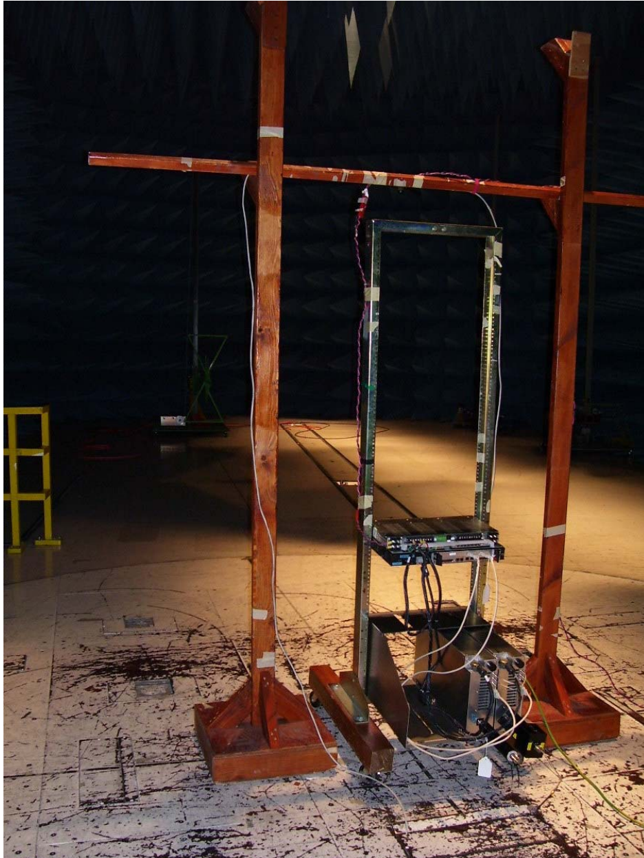
Radiated Emissions
