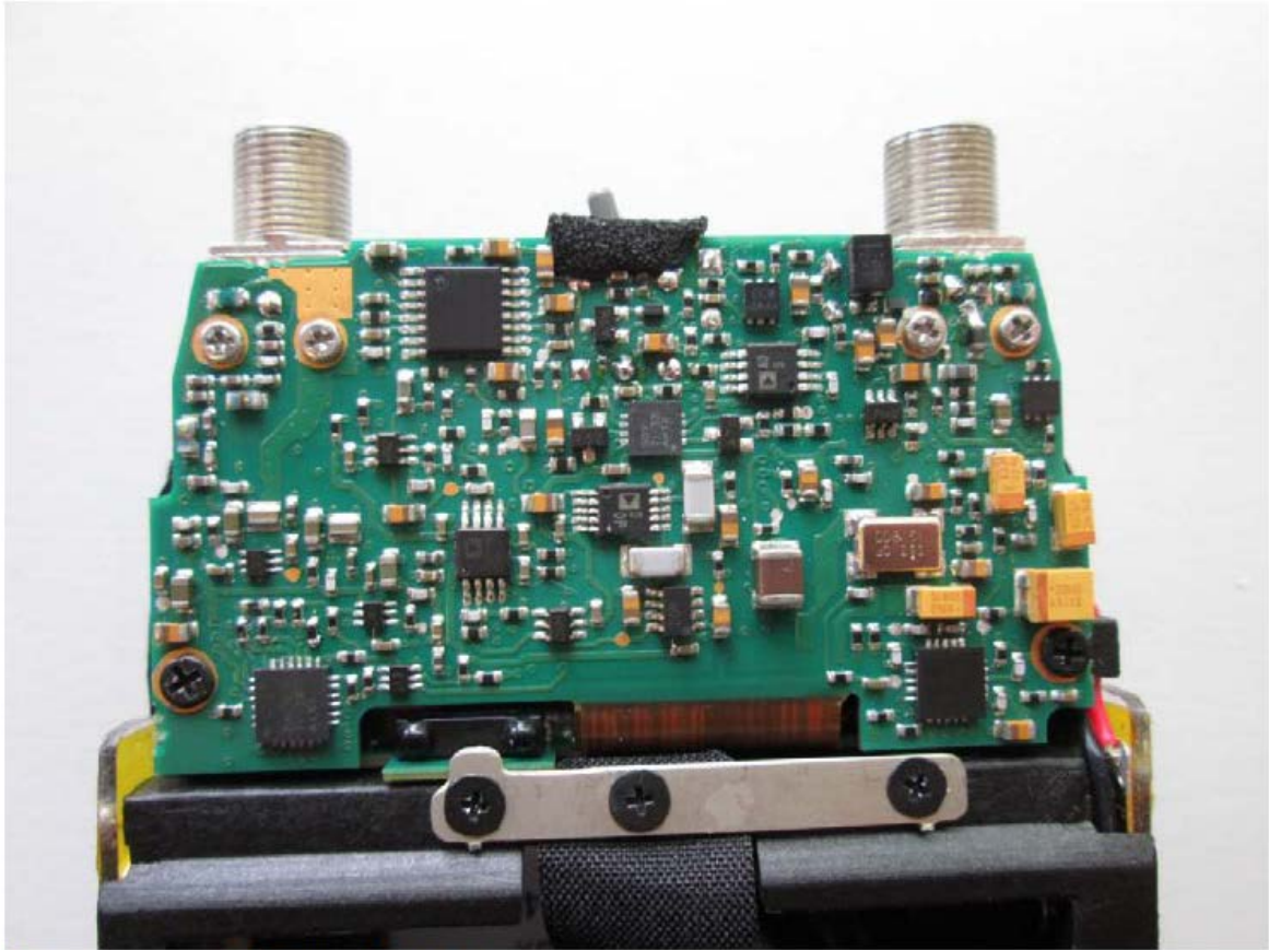
Main board of EUT #T1541593, bottom
