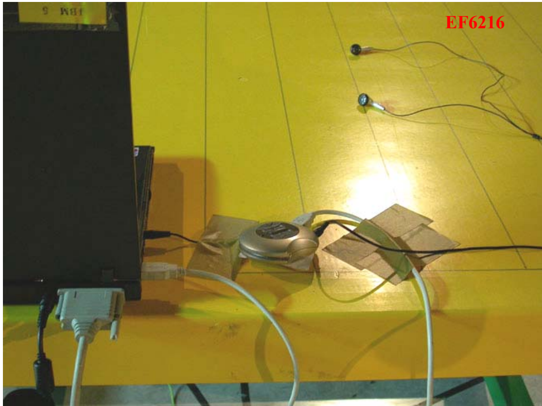
Photo 4: Spurious Emission Test Set-up photo
