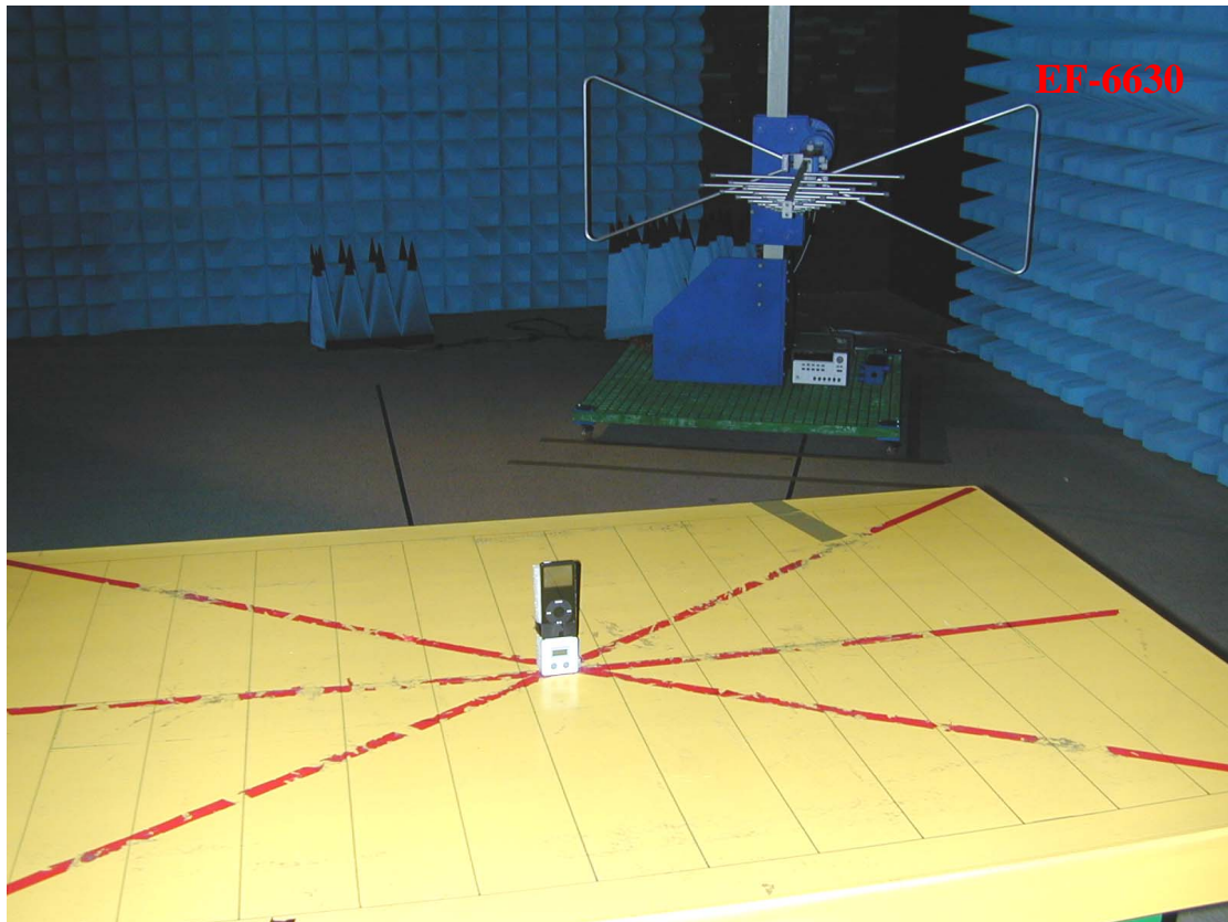
Photo 1: Spurious Emission Test Set-up photo
