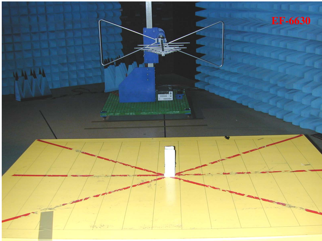
Photo 2: Spurious Emission Test Set-up photo
