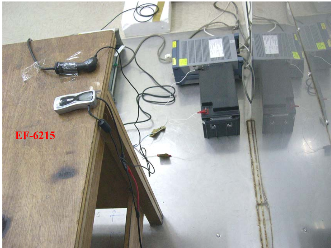
Photo 2: Conducted Emission Test Set-up
