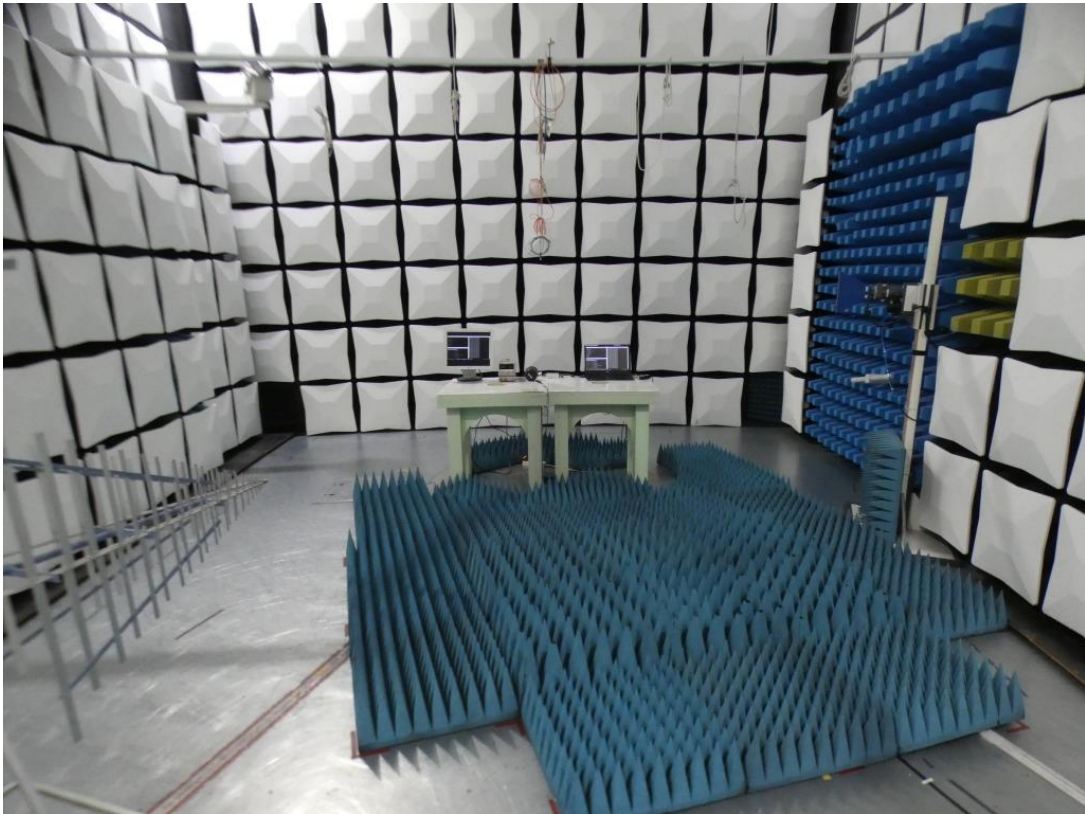
Photo 2: Test setup for radiated measurements FCC15b, above 1 GHz
