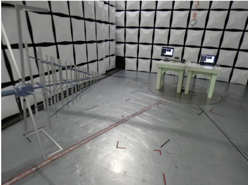
Photo 1: Test setup for radiated measurements FCC15b, below 1 GHz
