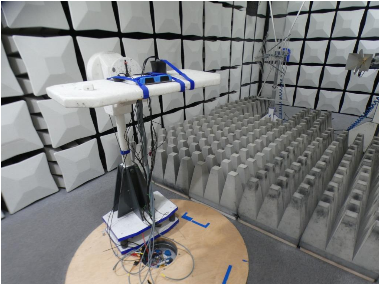
Photo 1: Test setup for radiated measurements, above 1 GHz
