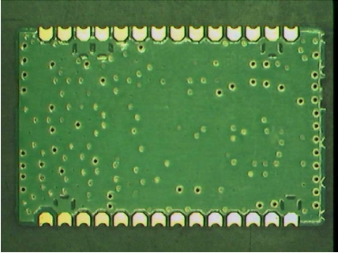
PCB buttom
