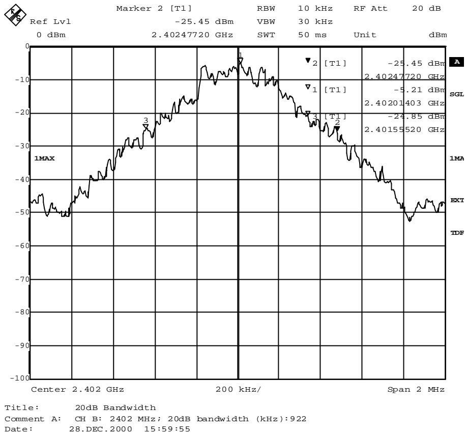
Occupied bandwidth (TX on 2402 MHz)
