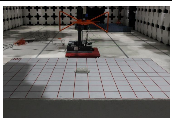
Radiated Emissions Rear (Below 1 GHz)
