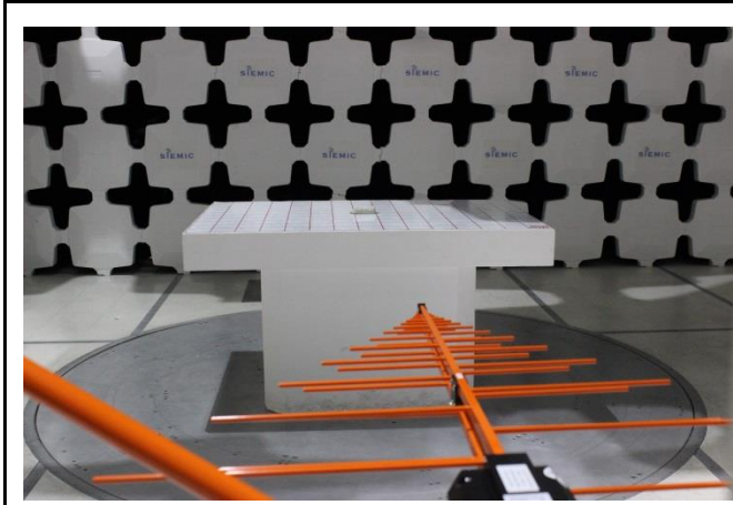
Radiated Emissions Front (Below 1 GHz)
