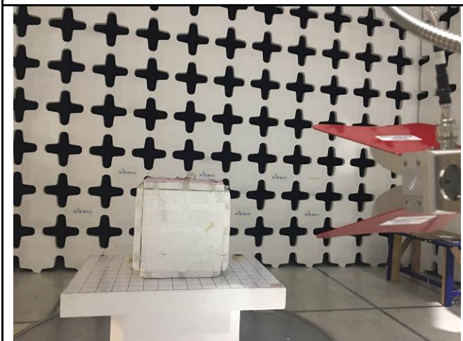
Radiated Emissions Front (Above 1 GHz)
