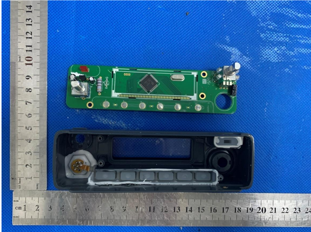
OPEN VIEW-4 OF EUT-1
