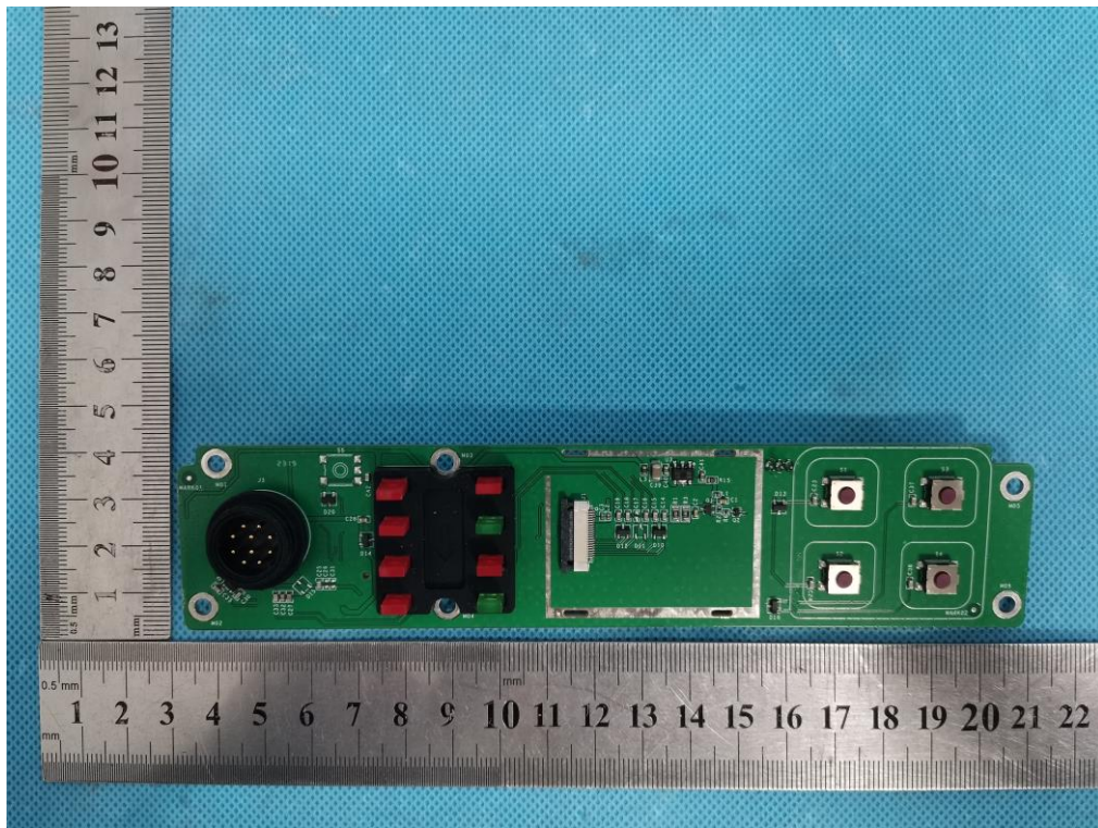
INTERNAL VIEW OF EUT (FIGURE 45)
