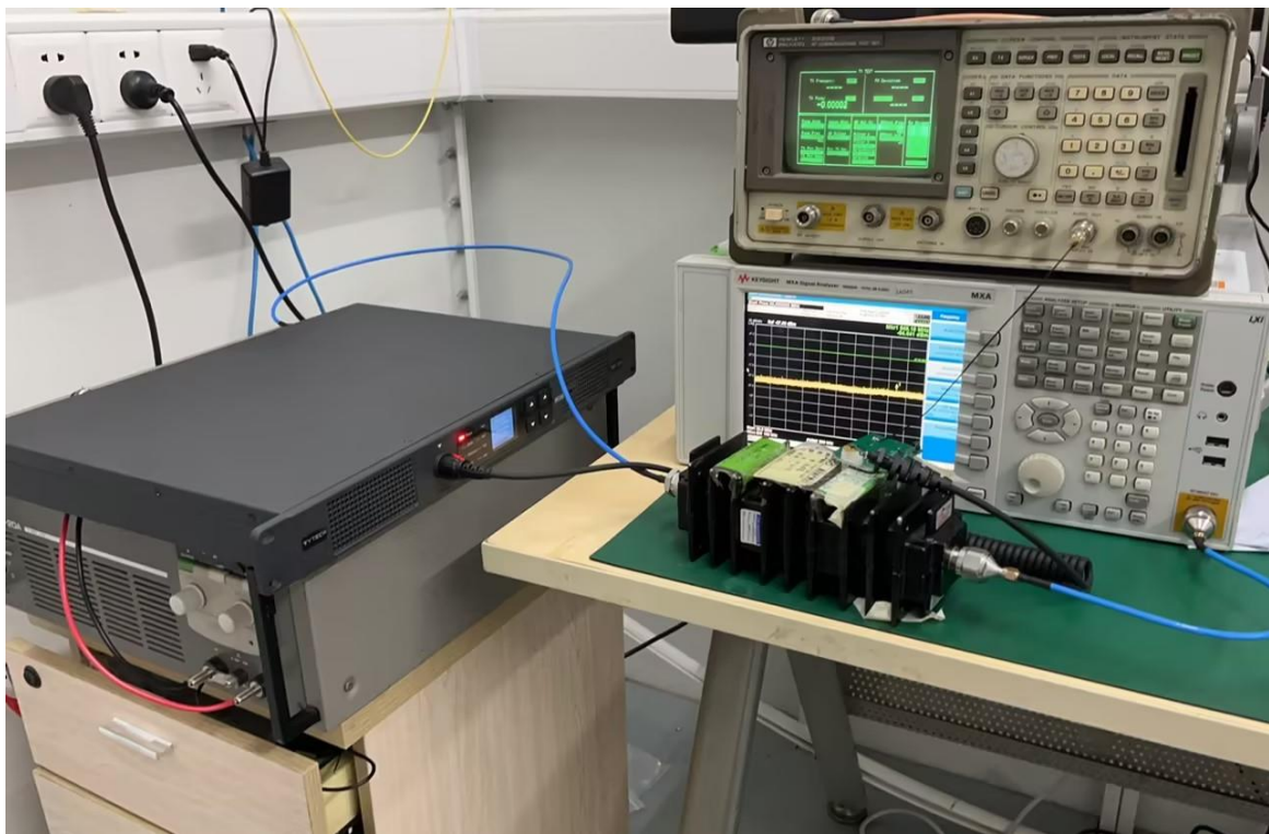
RF CONDUCTED TEST SETUP BY DC
