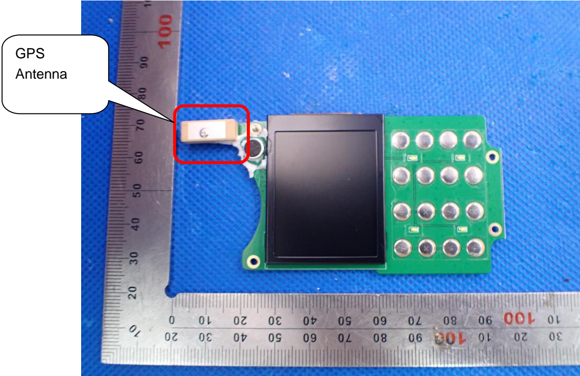
INTERNAL VIEW OF EUT(FIGURE 9)
