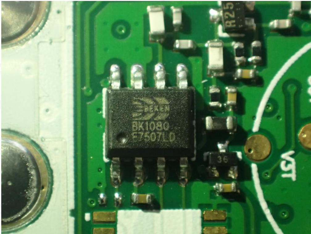
Part 2 TOP VIEW OF EUT
