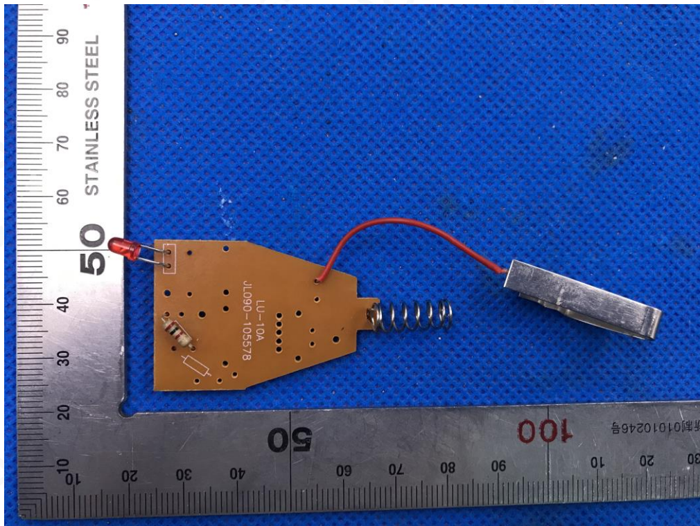
Part 3 TOP VIEW OF EUT
