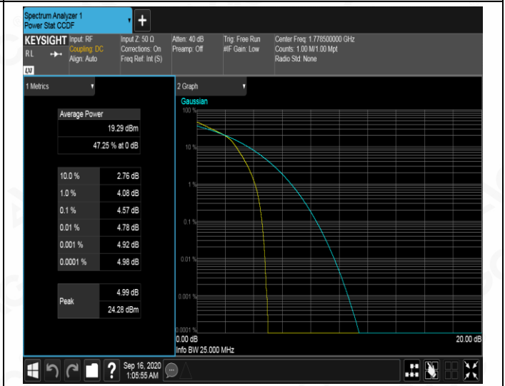
HCH_16QAM_15RB#0
