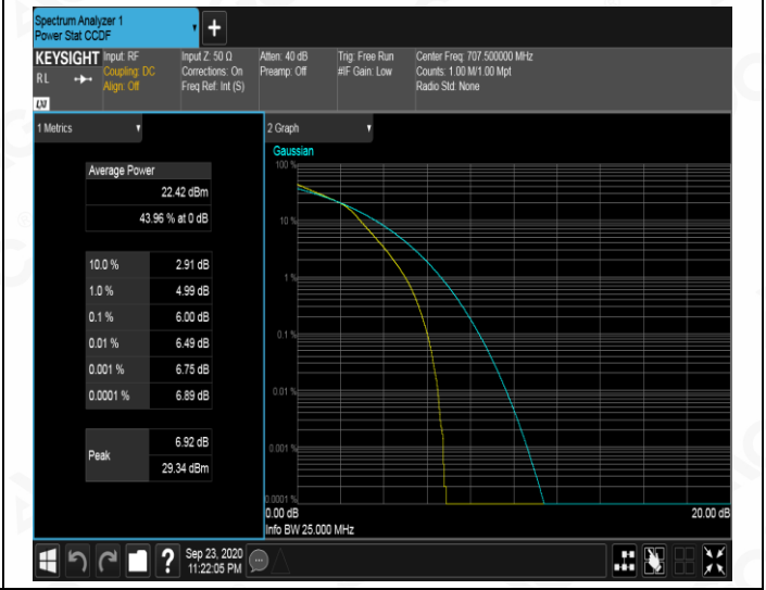
MCH_16QAM_15RB#0
