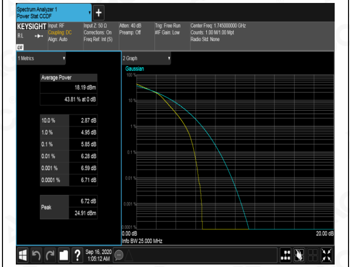
MCH_16QAM_15RB#0
