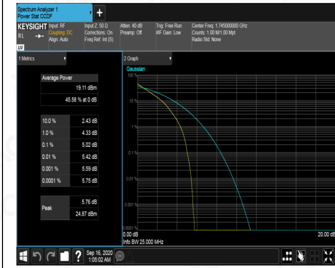
MCH_QPSK_15RB#0
