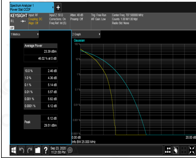
MCH_QPSK_15RB#0
