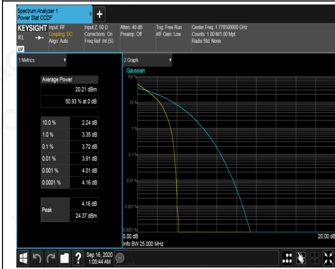
HCH_QPSK_15RB#0
