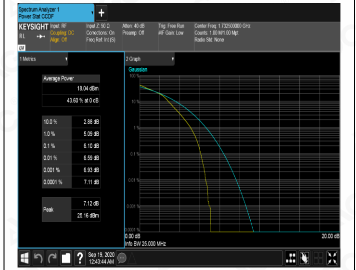
MCH_16QAM_15RB#0
