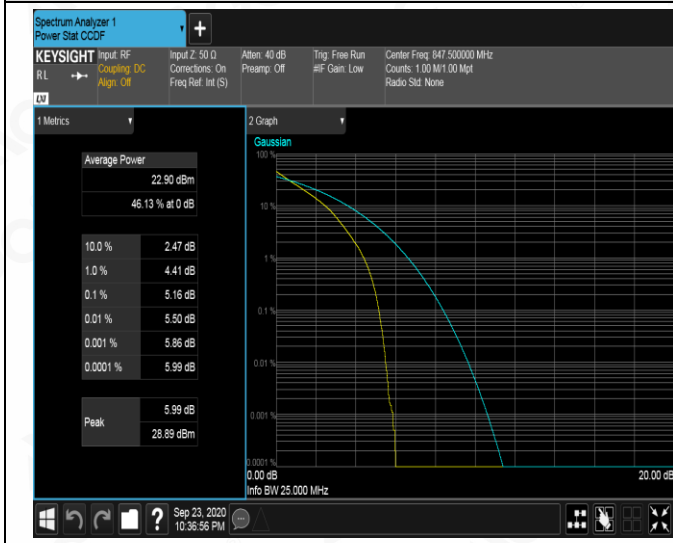
HCH_QPSK_15RB#0
