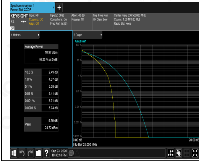
MCH_QPSK_15RB#0
